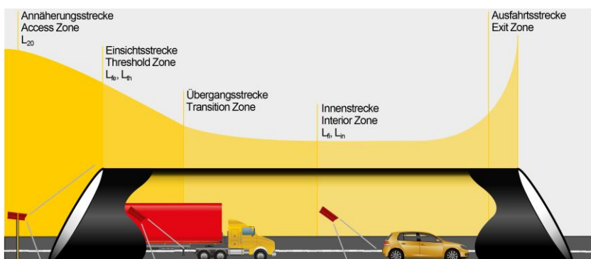
Measured luminances in a tunnel and locations of photometers
